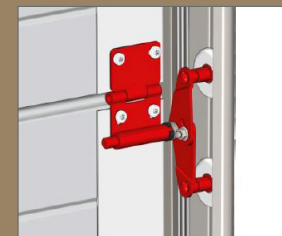
DOUBLES GALETS DE GUIDAGE
